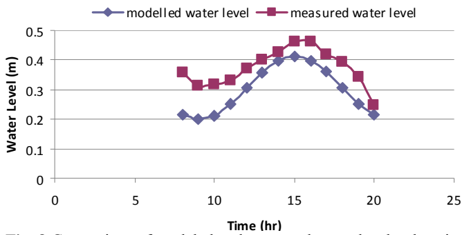
Fig. 8 Comparison of modeled and measured water level at location 2 (day 1).
