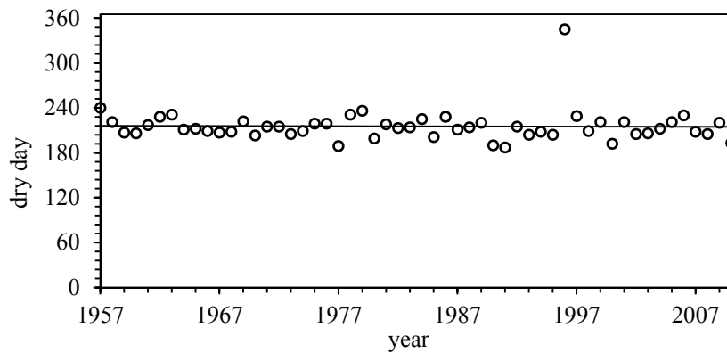
Fig. 4 Variation of annual dry days at Sylhet station for 1957 – 2010.
