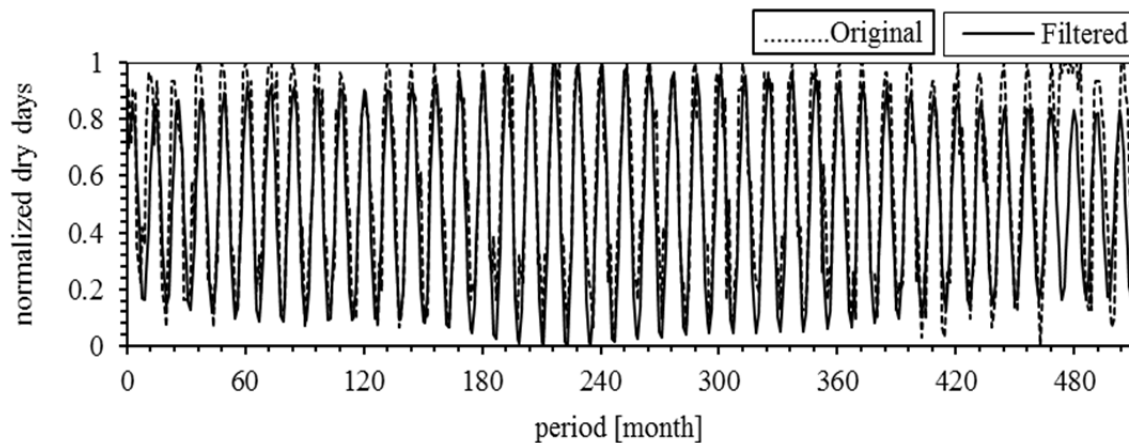
Fig. 8 Comparison between original monthly dry days variation and filtered (with a band pass filter 0.08 to 0.088 \text{month}^{-1} ) variation. Both the data series were normalized between 0 and 1 by the difference of the maximum and minimum values.
