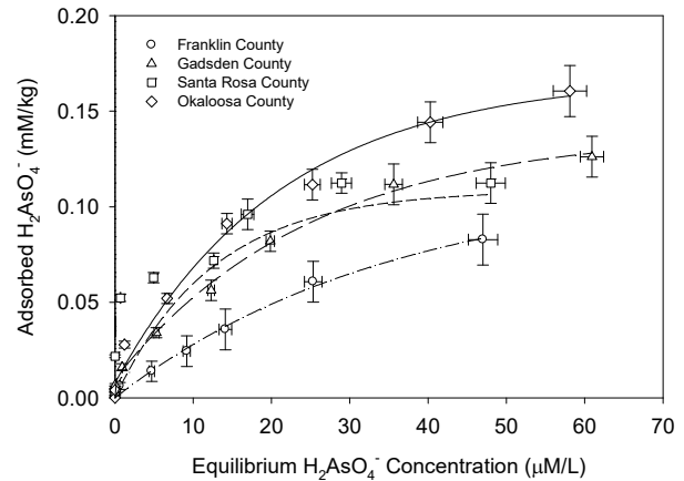
Fig. 1 As(V) Adsorption Isotherms in Landfill Soils.
