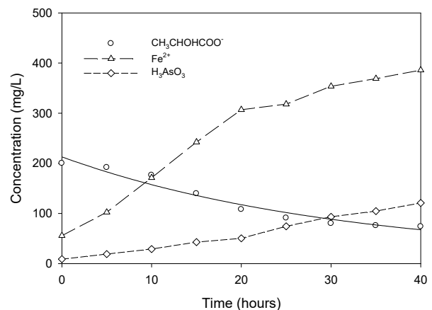
Fig. 2c Lactate Reduction and Fe(II) and As(III) Release in Santa Rosa County Landfill Soils.
