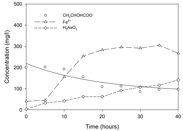
Fig. 2a Lactate Reduction and Fe(II) and As(III) Release in Franklin Landfill Soils.
