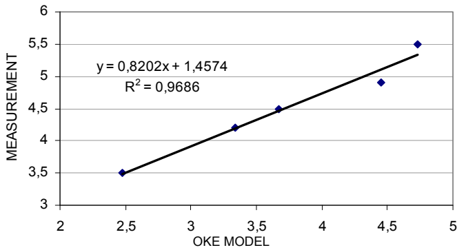
Fig 5. Measuring data × Oke model equation and coefficient of determination (R²).
