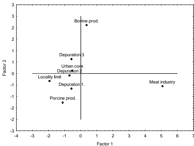
Fig. 2 Results of the Principal Components Analysis (PCA) based on values of physic-chemical variables and nutrients measured in winter sampling - Salado River-Argentina.
