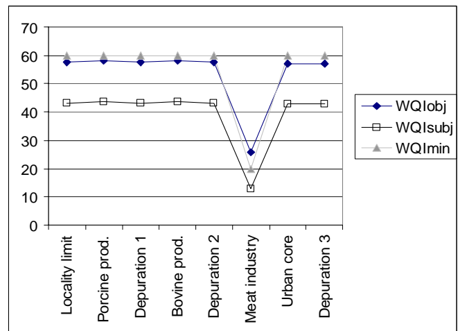
Fig. 4a Water quality indexes in winter sampling in Salado River.
