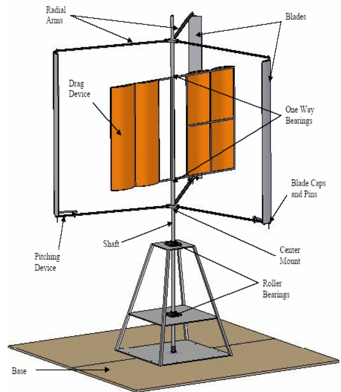
Fig. 4 Final assembly of the prototype wind turbine.
