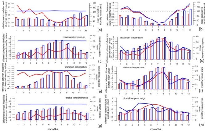
Fig. 7 Left column: continuous line ratio (first, difference (the other ones) between bias corrected (blue) or raw RCM (red) and observed value; absolute values are displayed as bars: (a) precipitation, (c) maximum temperature, (e) minimum temperature, (g) diurnal temporal range; Right column: continuous line ratio (first, difference (the other ones) between bias corrected (blue) or raw RCM (red) on future time span 2071-2100 (under RCP8.5) and control period 1981-2010; absolute values are displayed as bars: (b) runoff clay soil, (d) runoff sandy soil, (f) potential evaporation, (h) actual evaporation clay soil, (l) actual evaporation sandy soil.
